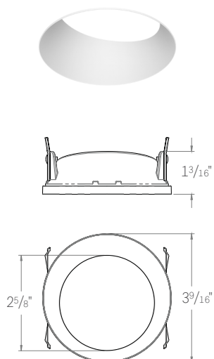
ED3-RATL ROUND ADJUSTABLE TRIMLESS
