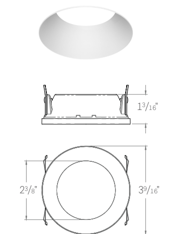
ED3-RFTL ROUND FIXED TRIMLESS Trimless Style for use with SAIC modules only.
