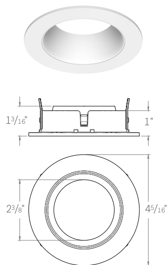
ED3-RFST ROUND FIXED STANDARD TRIM
