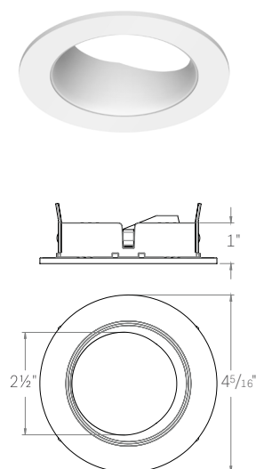
ED3-RAST ROUND ADJUSTABLE STANDARD TRIM
