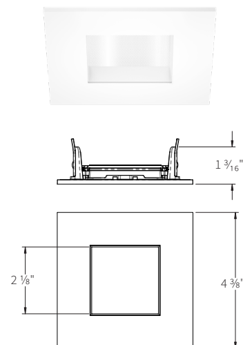
ED3-SAWR SQUARE ADJUSTABLE WET LOCATION REGRESSED
