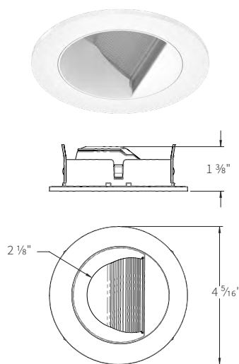
ED3-RFWW2 ROUND FIXED WALL WASH
