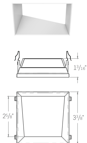
ED3-SATL SQUARE ADJUSTABLE TRIMLESS Adjustable trim styles for use with adjustable SAIC models only.
