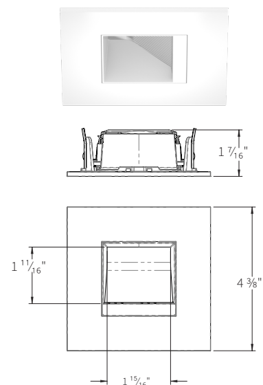
ED3-SFWW2 SQUARE FIXED WALL WASH
